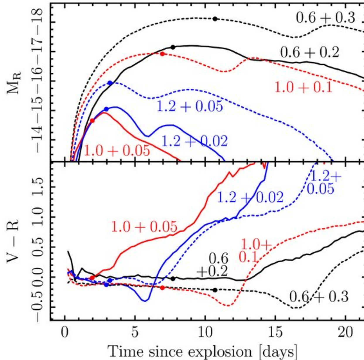
Figure 6. from Thermonuclear .Ia Supernovae from Helium Shell Detonations: Explosion Models and Observables SHEN ET AL. 2010 ApJ 715 767 doi:10.1088/0004-637X/715/2/767 https://dx.doi.org/10.1088/0004-637X/715/2/767 © 2010. The American Astronomical Society. All rights reserved.
