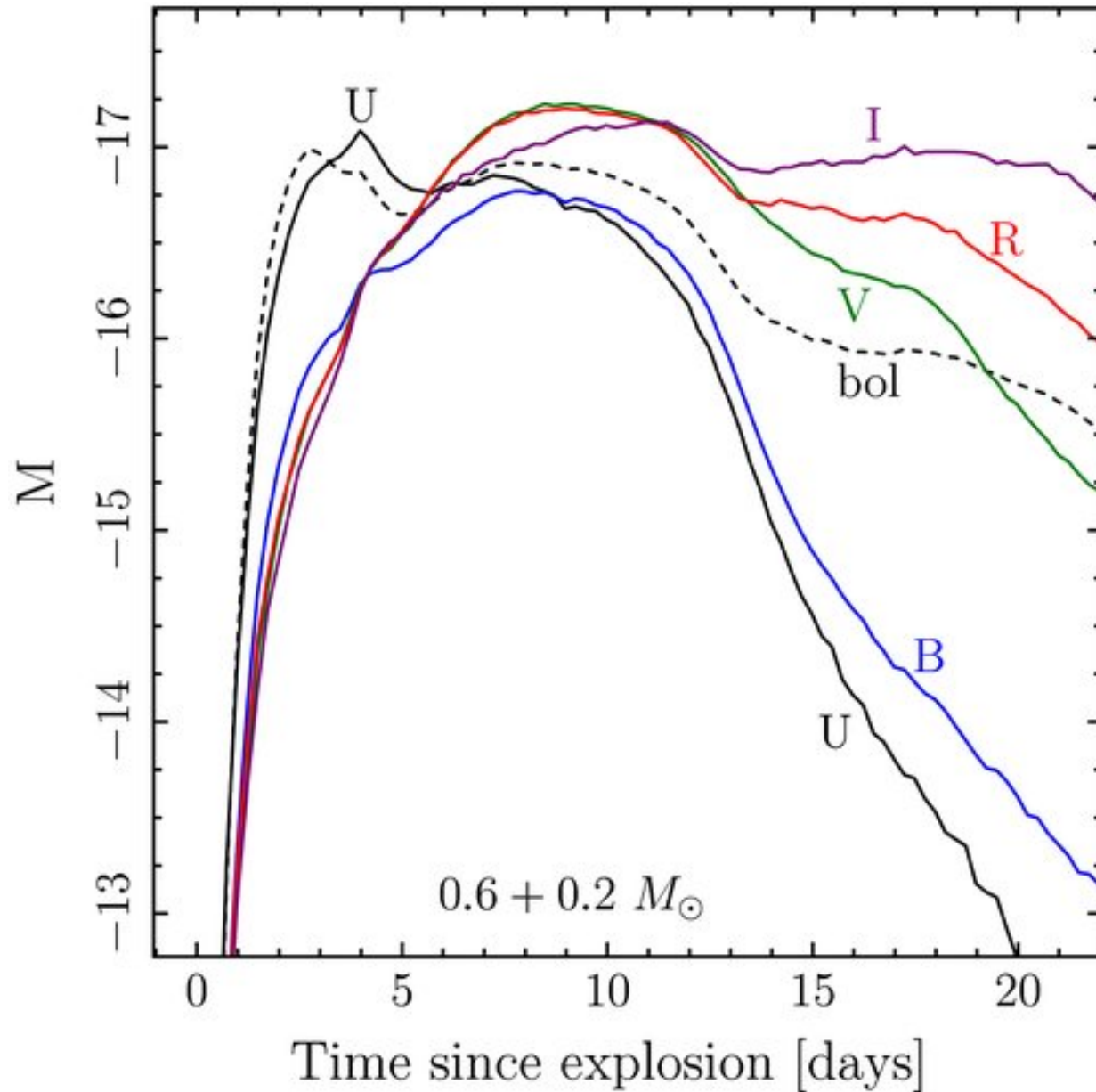
Figure 5. from Thermonuclear .Ia Supernovae from Helium Shell Detonations: Explosion Models and Observables SHEN ET AL. 2010 ApJ 715 767 doi:10.1088/0004-637X/715/2/767 https://dx.doi.org/10.1088/0004-637X/715/2/767 © 2010. The American Astronomical Society. All rights reserved.
