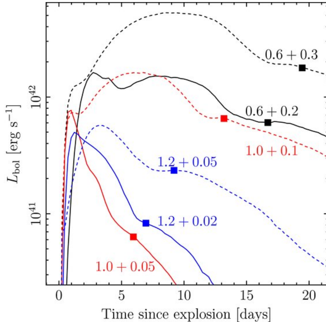
Figure 4. from Thermonuclear .Ia Supernovae from Helium Shell Detonations: Explosion Models and Observables SHEN ET AL. 2010 ApJ 715 767 doi:10.1088/0004-637X/715/2/767 https://dx.doi.org/10.1088/0004-637X/715/2/767 © 2010. The American Astronomical Society. All rights reserved.
