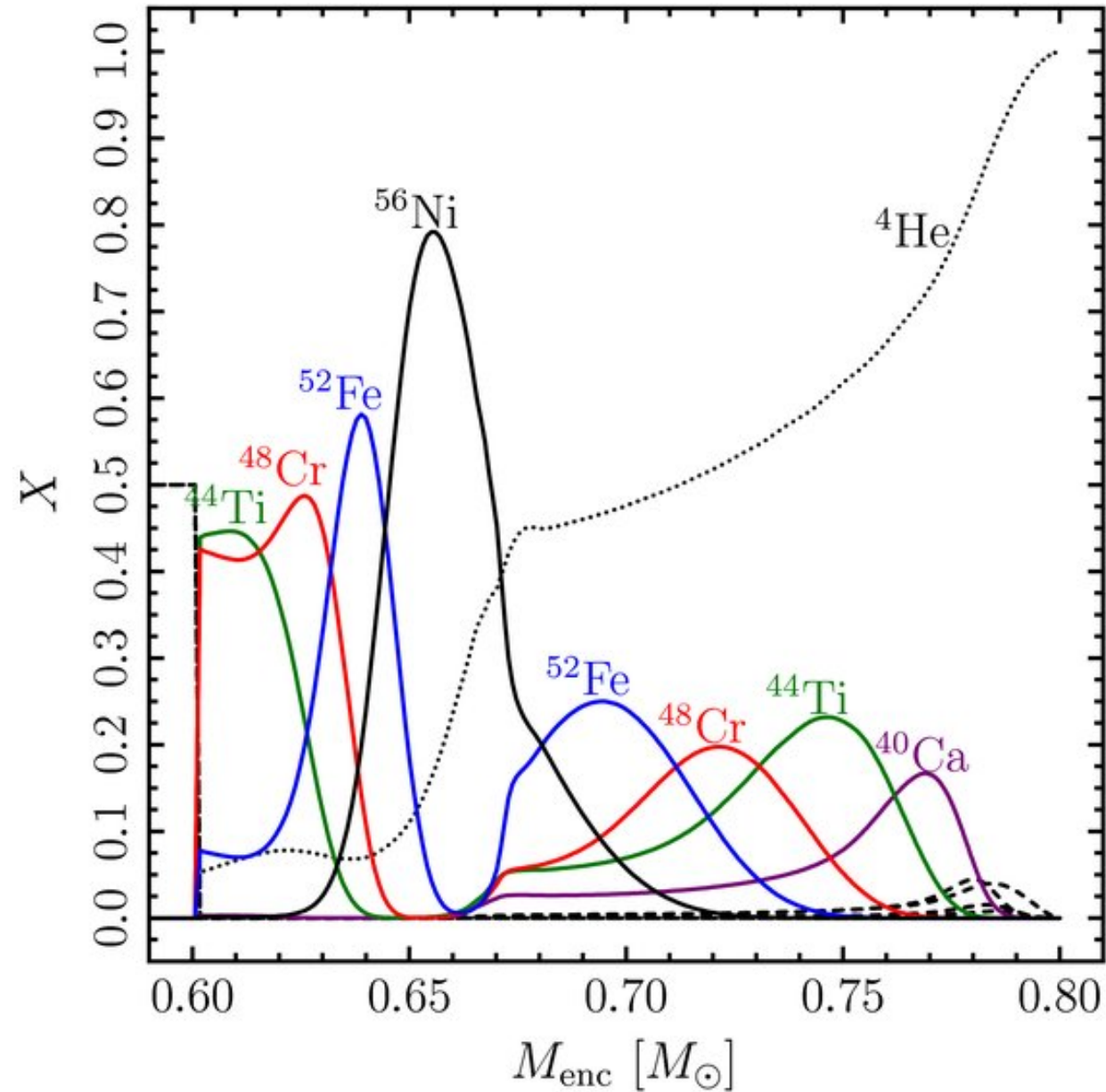
Figure 3. from Thermonuclear .Ia Supernovae from Helium Shell Detonations: Explosion Models and Observables SHEN ET AL. 2010 ApJ 715 767 doi:10.1088/0004-637X/715/2/767 https://dx.doi.org/10.1088/0004-637X/715/2/767 © 2010. The American Astronomical Society. All rights reserved.
