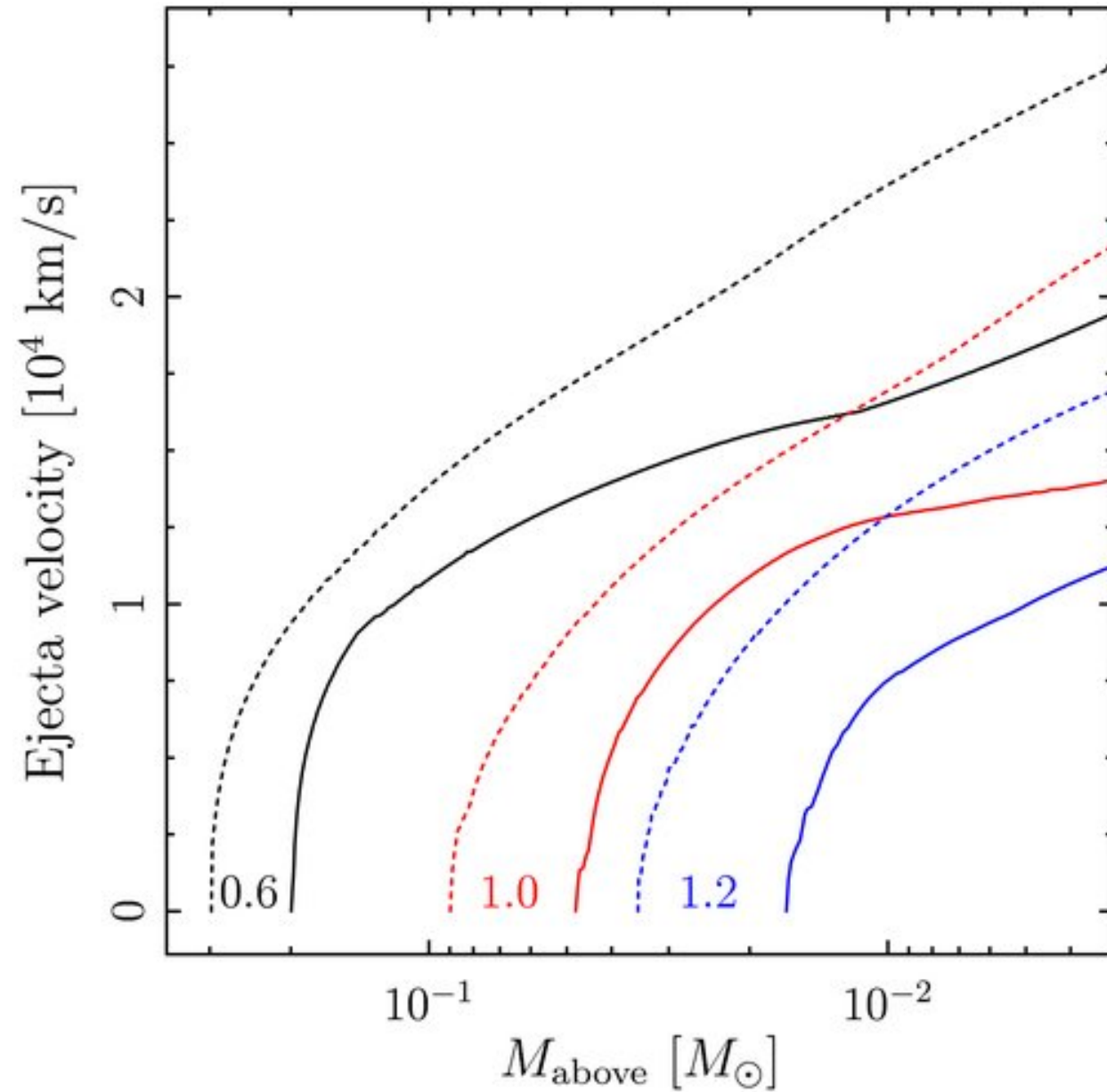
Figure 2. from Thermonuclear .Ia Supernovae from Helium Shell Detonations: Explosion Models and Observables SHEN ET AL. 2010 ApJ 715 767 doi:10.1088/0004-637X/715/2/767 https://dx.doi.org/10.1088/0004-637X/715/2/767 © 2010. The American Astronomical Society. All rights reserved.
