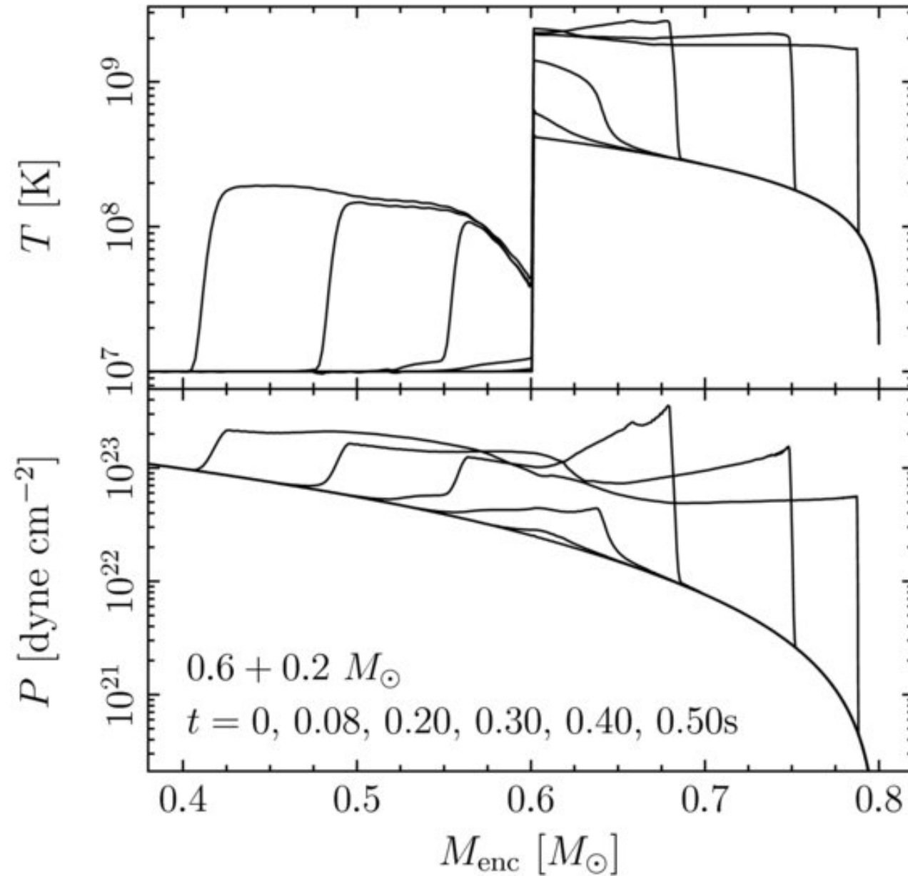
Figure 1. from Thermonuclear .Ia Supernovae from Helium Shell Detonations: Explosion Models and Observables SHEN ET AL. 2010 ApJ 715 767 doi:10.1088/0004-637X/715/2/767 https://dx.doi.org/10.1088/0004-637X/715/2/767 © 2010. The American Astronomical Society. All rights reserved.
