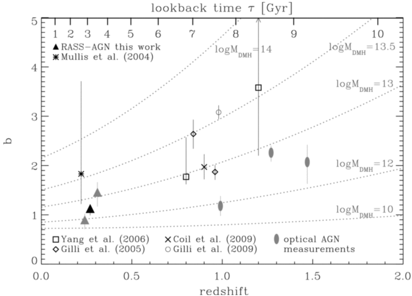
Figure 9. from The Spatial Clustering of ROSAT All-Sky Survey AGNs. I. The Cross-correlation Function with SDSS Luminous Red Galaxies KRUMPE, MIYAJI, & COIL 2010 ApJ 713 558 doi:10.1088/0004-637X/713/1/558 https://dx.doi.org/10.1088/0004-637X/713/1/558 © 2010. The American Astronomical Society. All rights reserved.
