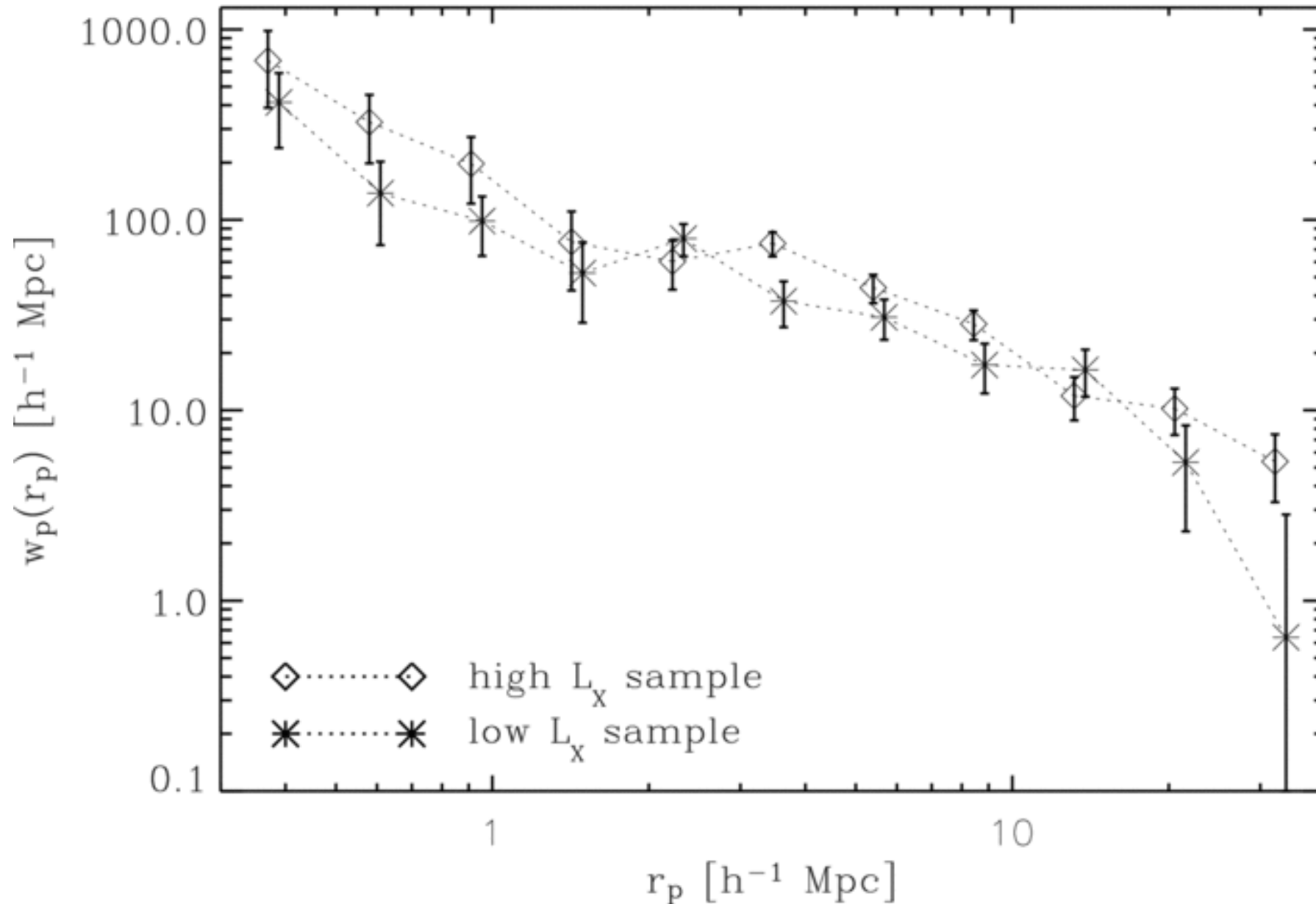
Figure 7. from The Spatial Clustering of ROSAT All-Sky Survey AGNs. I. The Cross-correlation Function with SDSS Luminous Red Galaxies KRUMPE, MIYAJI, & COIL 2010 ApJ 713 558 doi:10.1088/0004-637X/713/1/558 https://dx.doi.org/10.1088/0004-637X/713/1/558 © 2010. The American Astronomical Society. All rights reserved.
