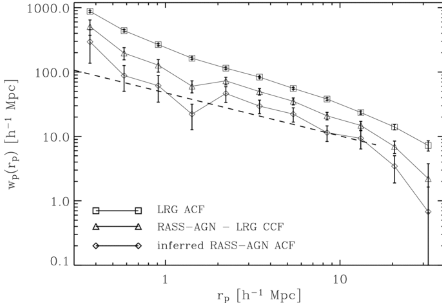
Figure 6. from The Spatial Clustering of ROSAT All-Sky Survey AGNs. I. The Cross-correlation Function with SDSS Luminous Red Galaxies KRUMPE, MIYAJI, & COIL 2010 ApJ 713 558 doi:10.1088/0004-637X/713/1/558 https://dx.doi.org/10.1088/0004-637X/713/1/558 © 2010. The American Astronomical Society. All rights reserved.
