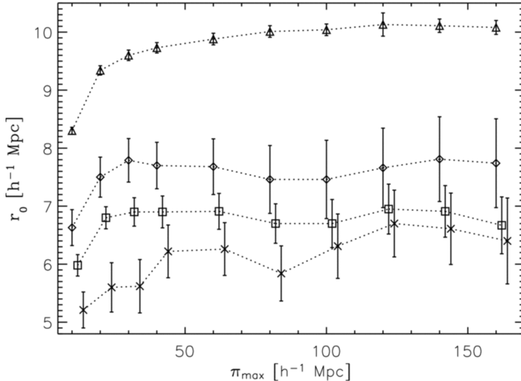
Figure 5. from The Spatial Clustering of ROSAT All-Sky Survey AGNs. I. The Cross-correlation Function with SDSS Luminous Red Galaxies KRUMPE, MIYAJI, & COIL 2010 ApJ 713 558 doi:10.1088/0004-637X/713/1/558 https://dx.doi.org/10.1088/0004-637X/713/1/558 © 2010. The American Astronomical Society. All rights reserved.
