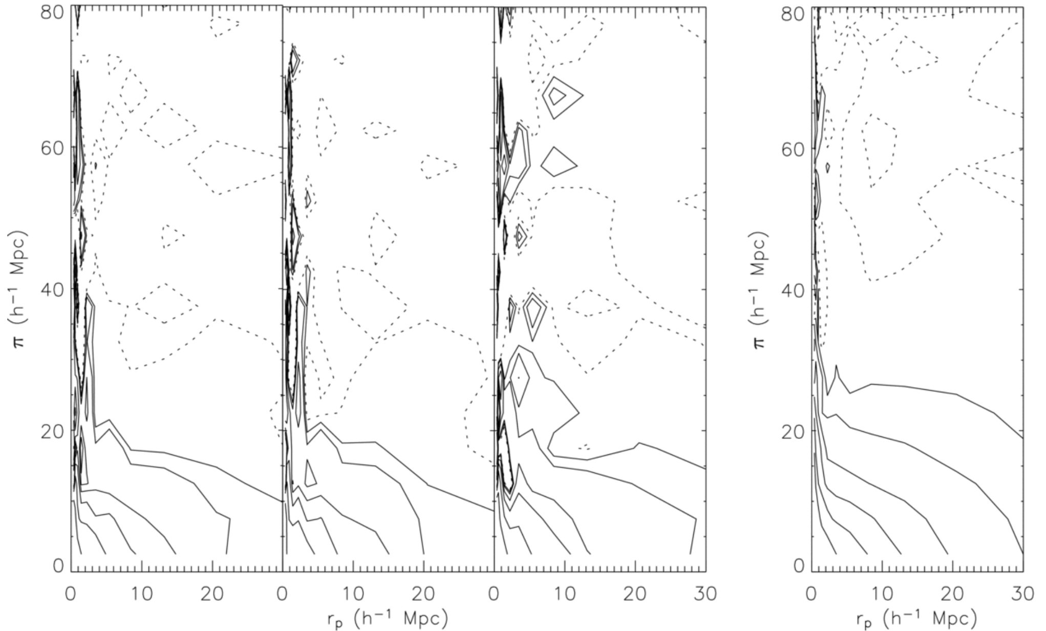
Figure 4. from The Spatial Clustering of ROSAT All-Sky Survey AGNs. I. The Cross-correlation Function with SDSS Luminous Red Galaxies KRUMPE, MIYAJI, & COIL 2010 ApJ 713 558 doi:10.1088/0004-637X/713/1/558 https://dx.doi.org/10.1088/0004-637X/713/1/558 © 2010. The American Astronomical Society. All rights reserved.
