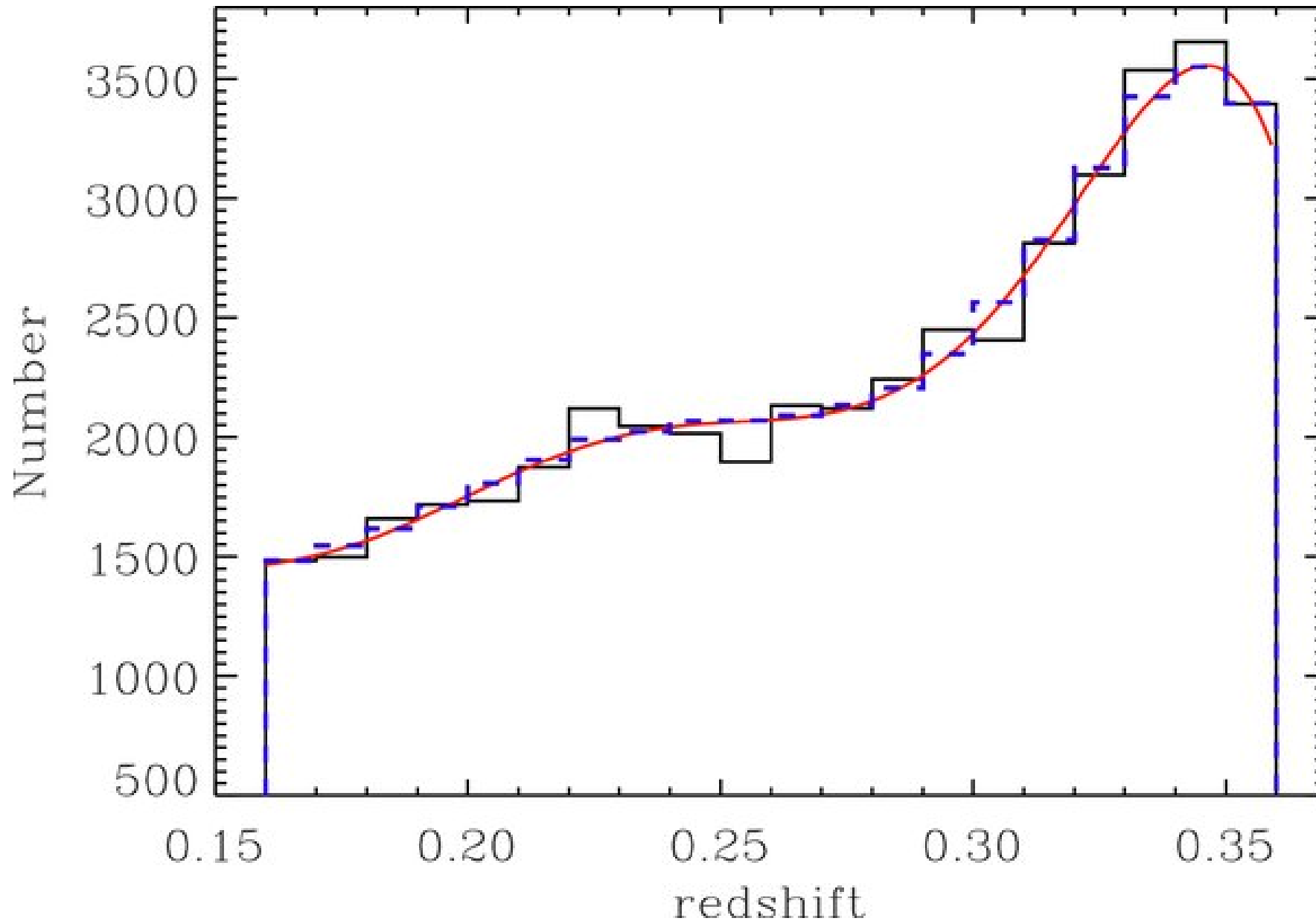
Figure 3. from The Spatial Clustering of ROSAT All-Sky Survey AGNs. I. The Cross-correlation Function with SDSS Luminous Red Galaxies KRUMPE, MIYAJI, & COIL 2010 ApJ 713 558 doi:10.1088/0004-637X/713/1/558 https://dx.doi.org/10.1088/0004-637X/713/1/558 © 2010. The American Astronomical Society. All rights reserved.
