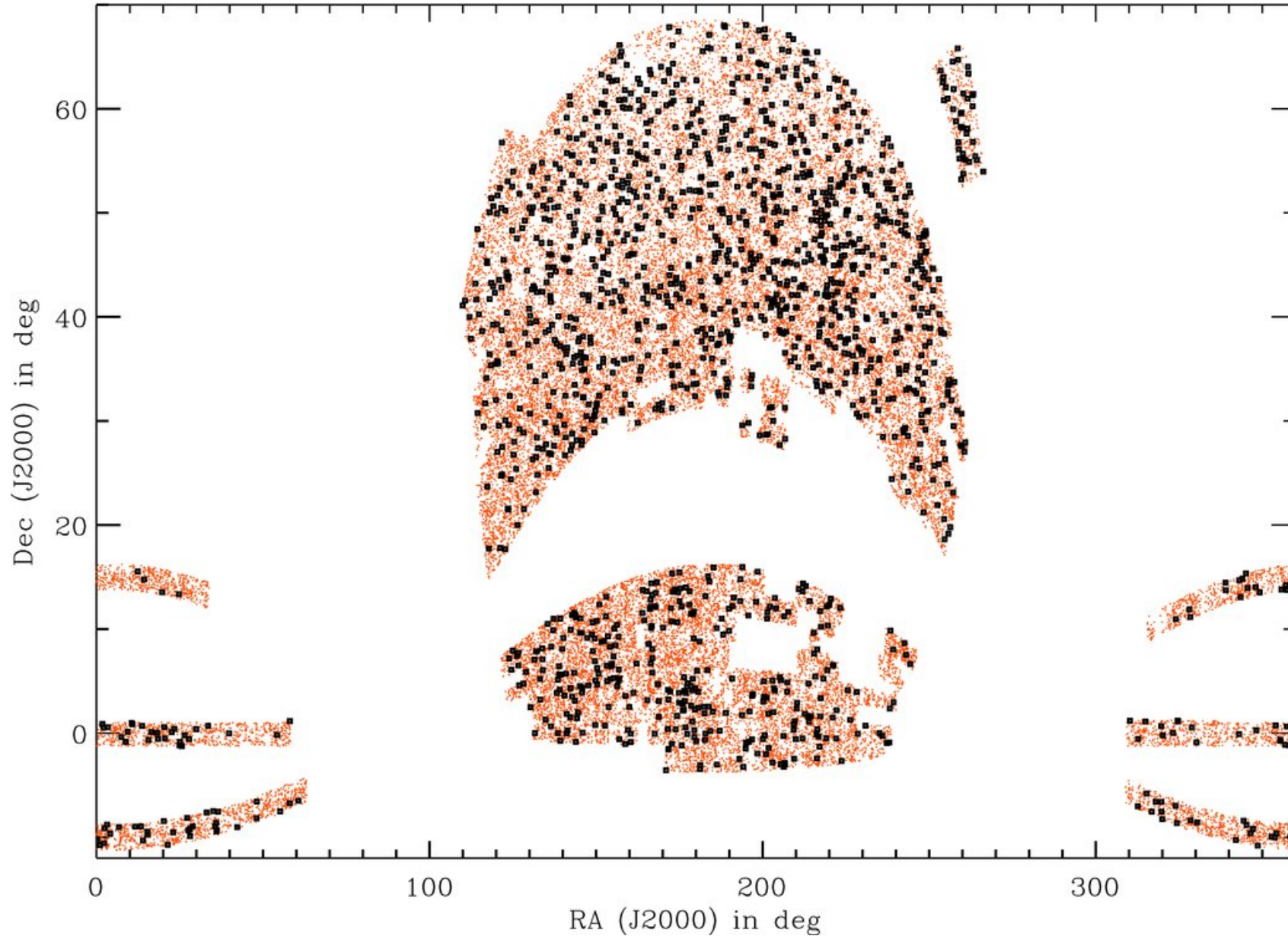
Figure 2. from The Spatial Clustering of ROSAT All-Sky Survey AGNs. I. The Cross-correlation Function with SDSS Luminous Red Galaxies KRUMPE, MIYAJI, & COIL 2010 ApJ 713 558 doi:10.1088/0004-637X/713/1/558 https://dx.doi.org/10.1088/0004-637X/713/1/558 © 2010. The American Astronomical Society. All rights reserved.
