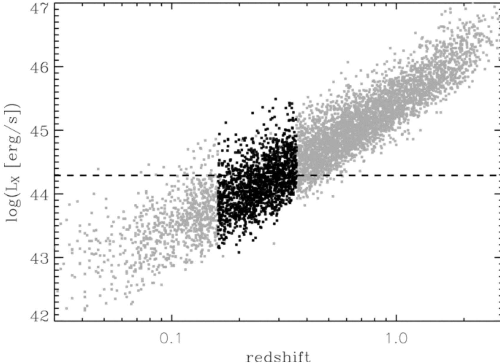
Figure 1. from The Spatial Clustering of ROSAT All-Sky Survey AGNs. I. The Cross-correlation Function with SDSS Luminous Red Galaxies KRUMPE, MIYAJI, & COIL 2010 ApJ 713 558 doi:10.1088/0004-637X/713/1/558 https://dx.doi.org/10.1088/0004-637X/713/1/558 © 2010. The American Astronomical Society. All rights reserved.
