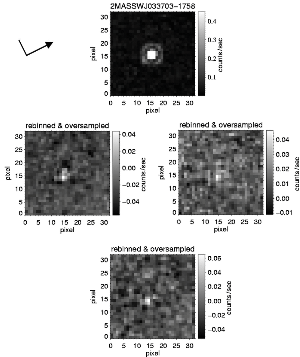
Figure 7. from The Search for Planetary Mass Companions to Field Brown Dwarfs with HST/NICMOS STUMPF ET AL. 2010 ApJ 724 1 doi:10.1088/0004-637X/724/1/1 https://dx.doi.org/10.1088/0004-637X/724/1/1 © 2010. The American Astronomical Society. All rights reserved.
