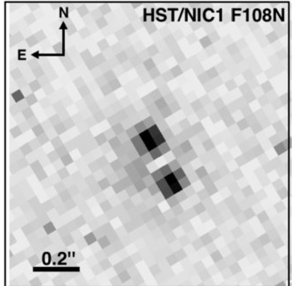
Figure 6. from The Search for Planetary Mass Companions to Field Brown Dwarfs with HST/NICMOS STUMPF ET AL. 2010 ApJ 724 1 doi:10.1088/0004-637X/724/1/1 https://dx.doi.org/10.1088/0004-637X/724/1/1 © 2010. The American Astronomical Society. All rights reserved.
