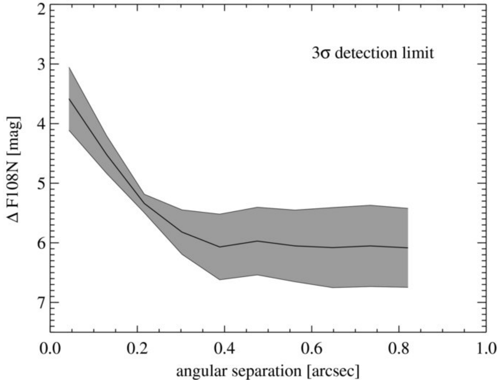
Figure 4. from The Search for Planetary Mass Companions to Field Brown Dwarfs with HST/NICMOS STUMPF ET AL. 2010 ApJ 724 1 doi:10.1088/0004-637X/724/1/1 https://dx.doi.org/10.1088/0004-637X/724/1/1 © 2010. The American Astronomical Society. All rights reserved.
