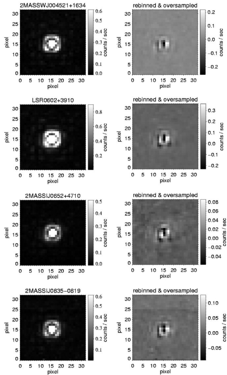
Figure 3. from The Search for Planetary Mass Companions to Field Brown Dwarfs with HST/NICMOS STUMPF ET AL. 2010 ApJ 724 1 doi:10.1088/0004-637X/724/1/1 https://dx.doi.org/10.1088/0004-637X/724/1/1
