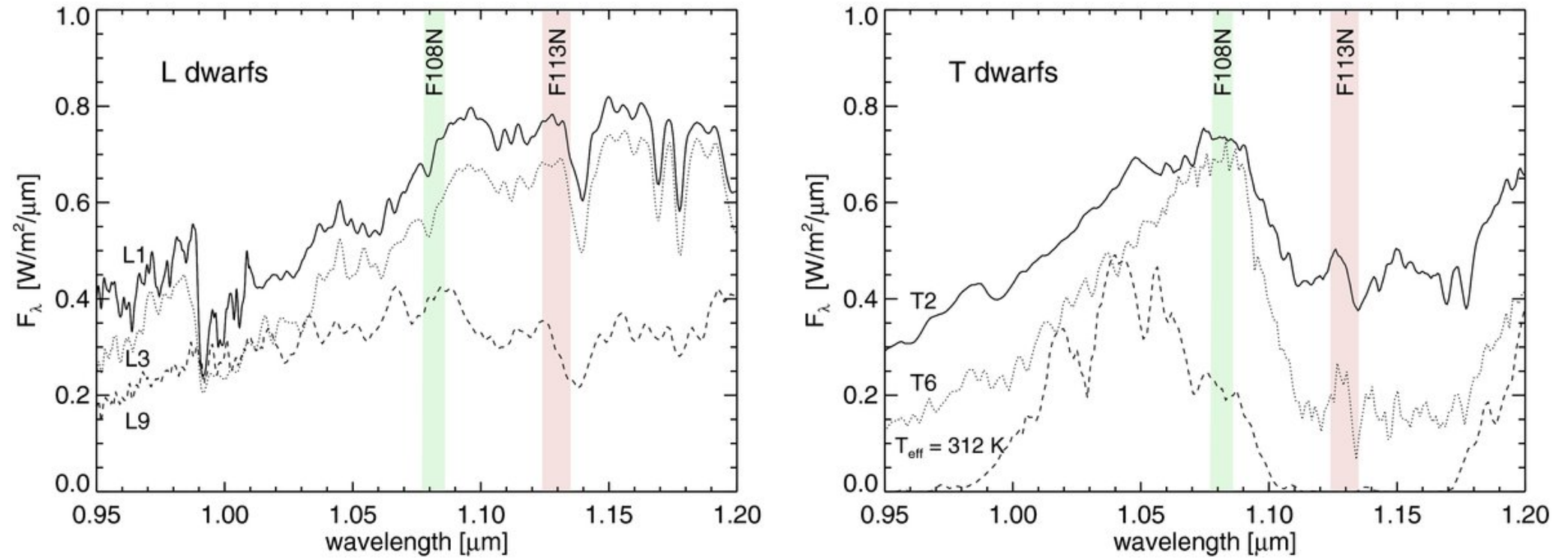
Figure 1. from The Search for Planetary Mass Companions to Field Brown Dwarfs with HST/NICMOS STUMPF ET AL. 2010 ApJ 724 1 doi:10.1088/0004-637X/724/1/1 https://dx.doi.org/10.1088/0004-637X/724/1/1 © 2010. The American Astronomical Society. All rights reserved.
