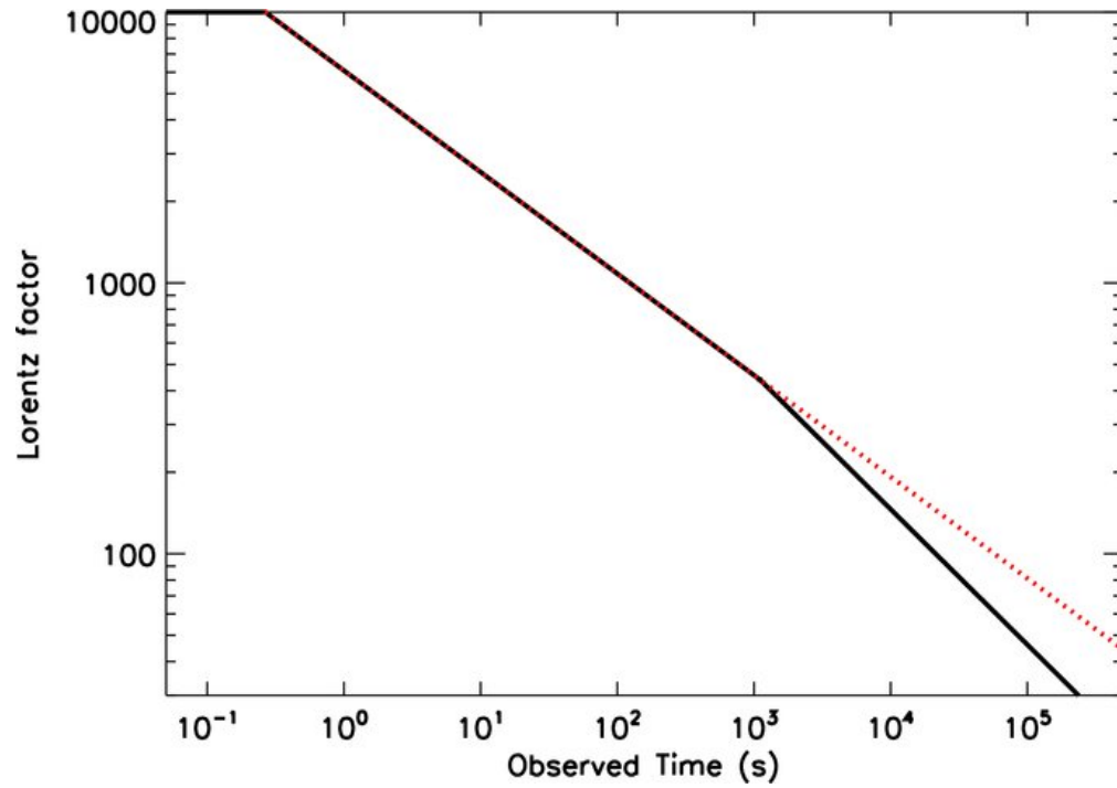
Figure 3. from High-energy Emission Components in the Short GRB 090510 CORSI, GUETTA, & PIRO 2010 ApJ 720 1008 doi:10.1088/0004-637X/720/2/1008 https://dx.doi.org/10.1088/0004-637X/720/2/1008 © 2010. The American Astronomical Society. All rights reserved.
