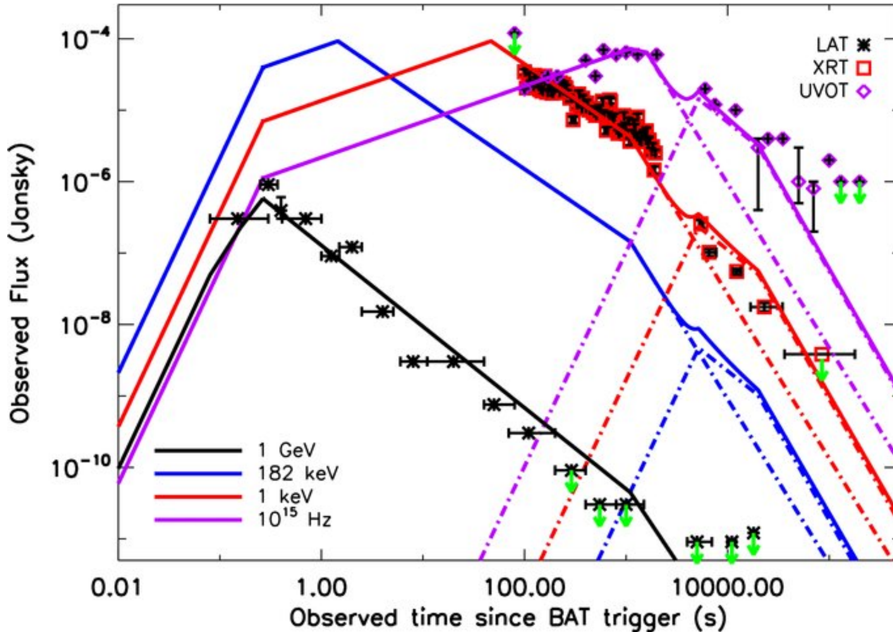
Figure 2. from High-energy Emission Components in the Short GRB 090510 CORSI, GUETTA, & PIRO 2010 ApJ 720 1008 doi:10.1088/0004-637X/720/2/1008 https://dx.doi.org/10.1088/0004-637X/720/2/1008 © 2010. The American Astronomical Society. All rights reserved.
