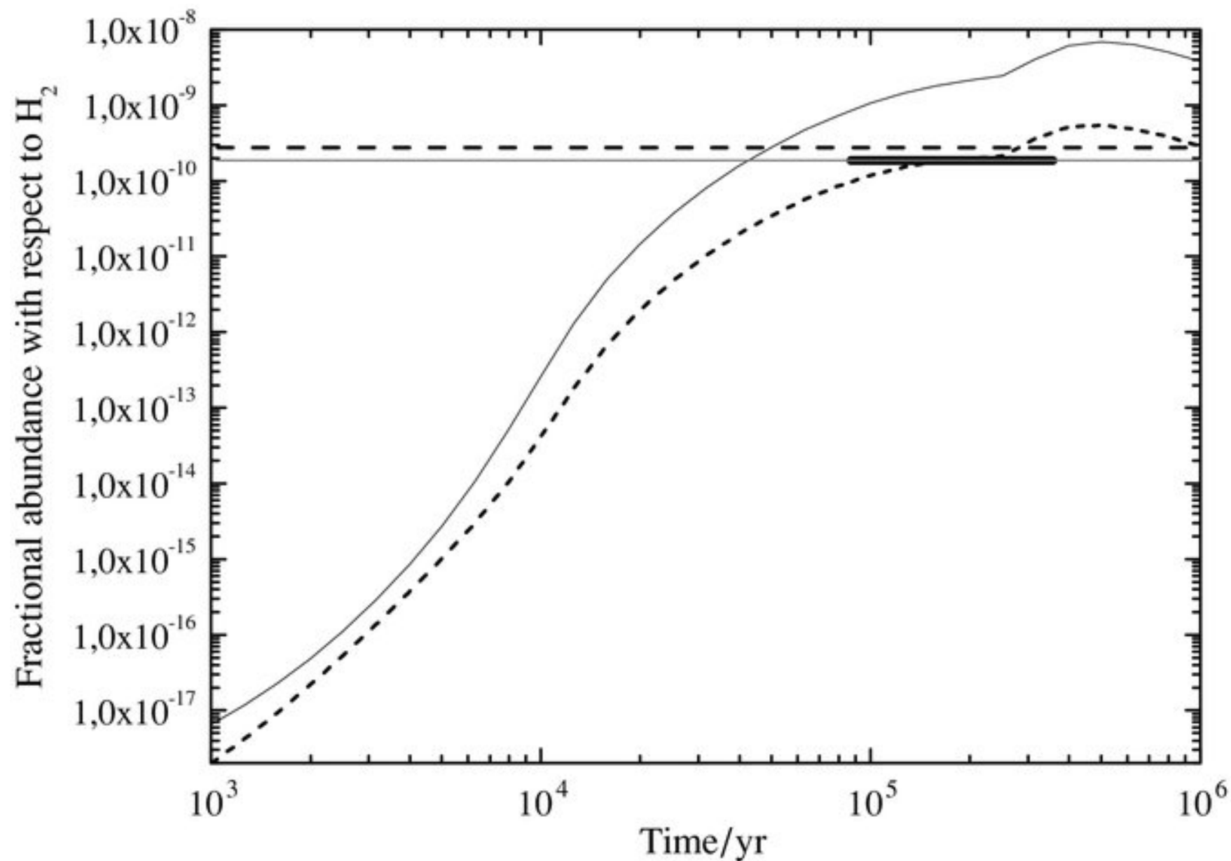
Figure 3. from Dissociative Recombination of Protonated Formic Acid: Implications for Molecular Cloud and Cometary Chemistry VIGREN ET AL. 2010 ApJ 709 1429 doi:10.1088/0004-637X/709/2/1429 https://dx.doi.org/10.1088/0004-637X/709/2/1429 © 2010. The American Astronomical Society. All rights reserved.
