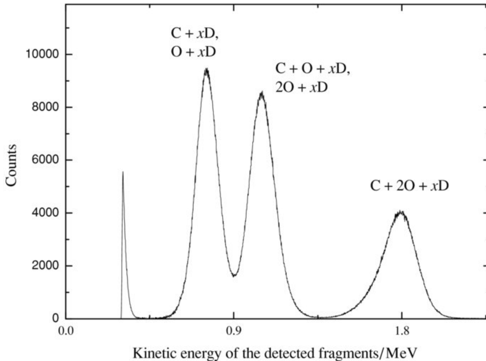
Figure 2. from Dissociative Recombination of Protonated Formic Acid: Implications for Molecular Cloud and Cometary Chemistry VIGREN ET AL. 2010 ApJ 709 1429 doi:10.1088/0004-637X/709/2/1429 https://dx.doi.org/10.1088/0004-637X/709/2/1429 © 2010. The American Astronomical Society. All rights reserved.
