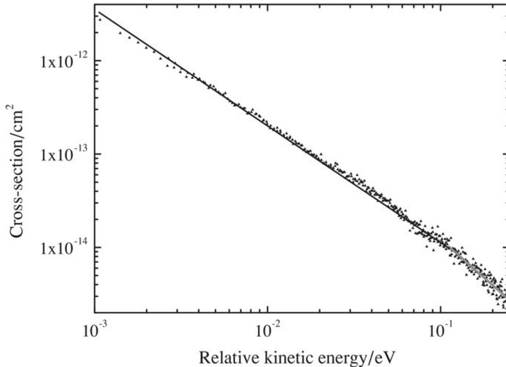
Figure 1. from Dissociative Recombination of Protonated Formic Acid: Implications for Molecular Cloud and Cometary Chemistry VIGREN ET AL. 2010 ApJ 709 1429 doi:10.1088/0004-637X/709/2/1429 https://dx.doi.org/10.1088/0004-637X/709/2/1429 © 2010. The American Astronomical Society. All rights reserved.
