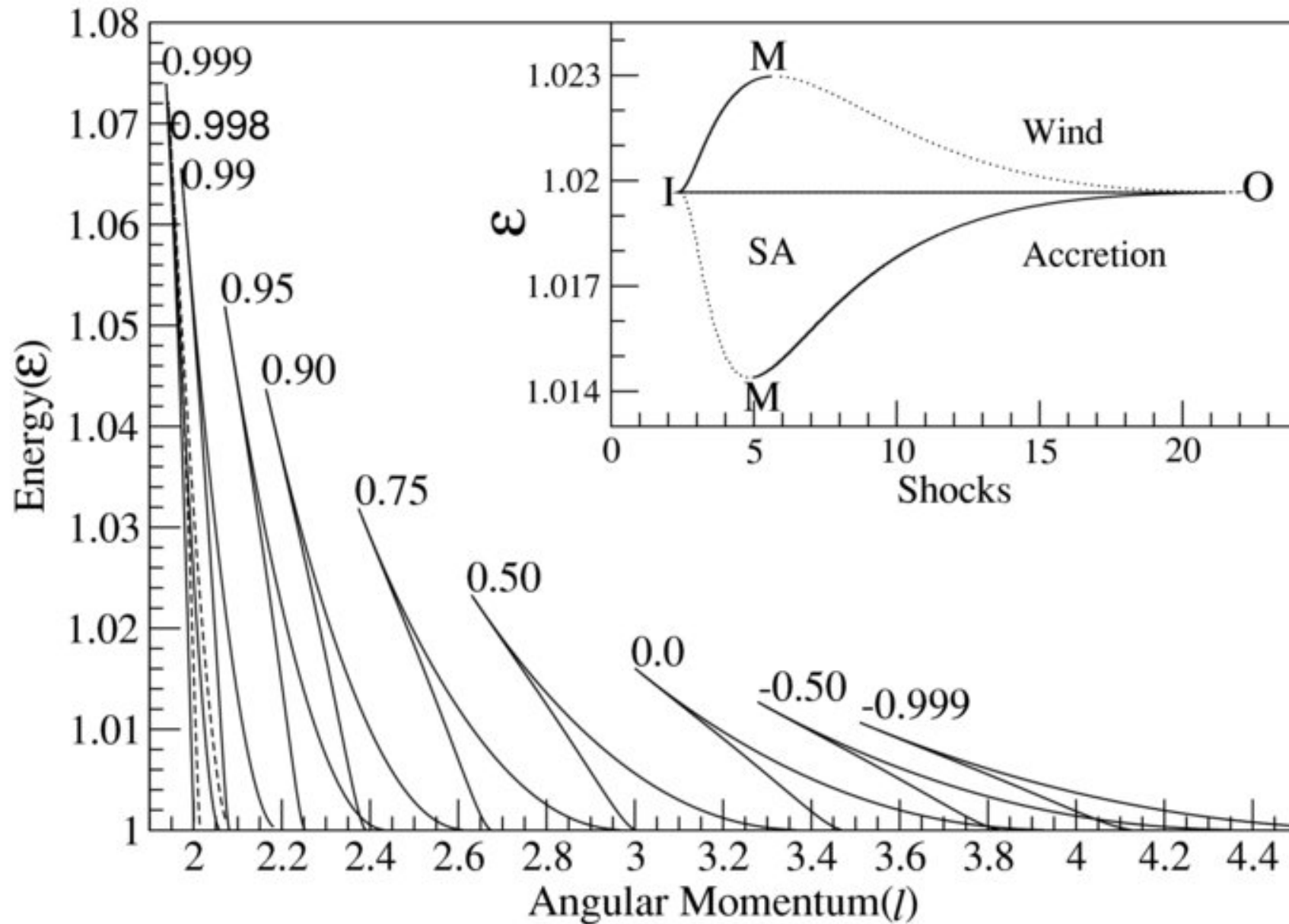
Figure 2. from Black Hole Mass and Spin from the 2:3 Twin-peak QPOs in Microquasars MONDAL 2010 ApJ 708 1442 doi:10.1088/0004-637X/708/2/1442 https://dx.doi.org/10.1088/0004-637X/708/2/1442 © 2010. The American Astronomical Society. All rights reserved.
