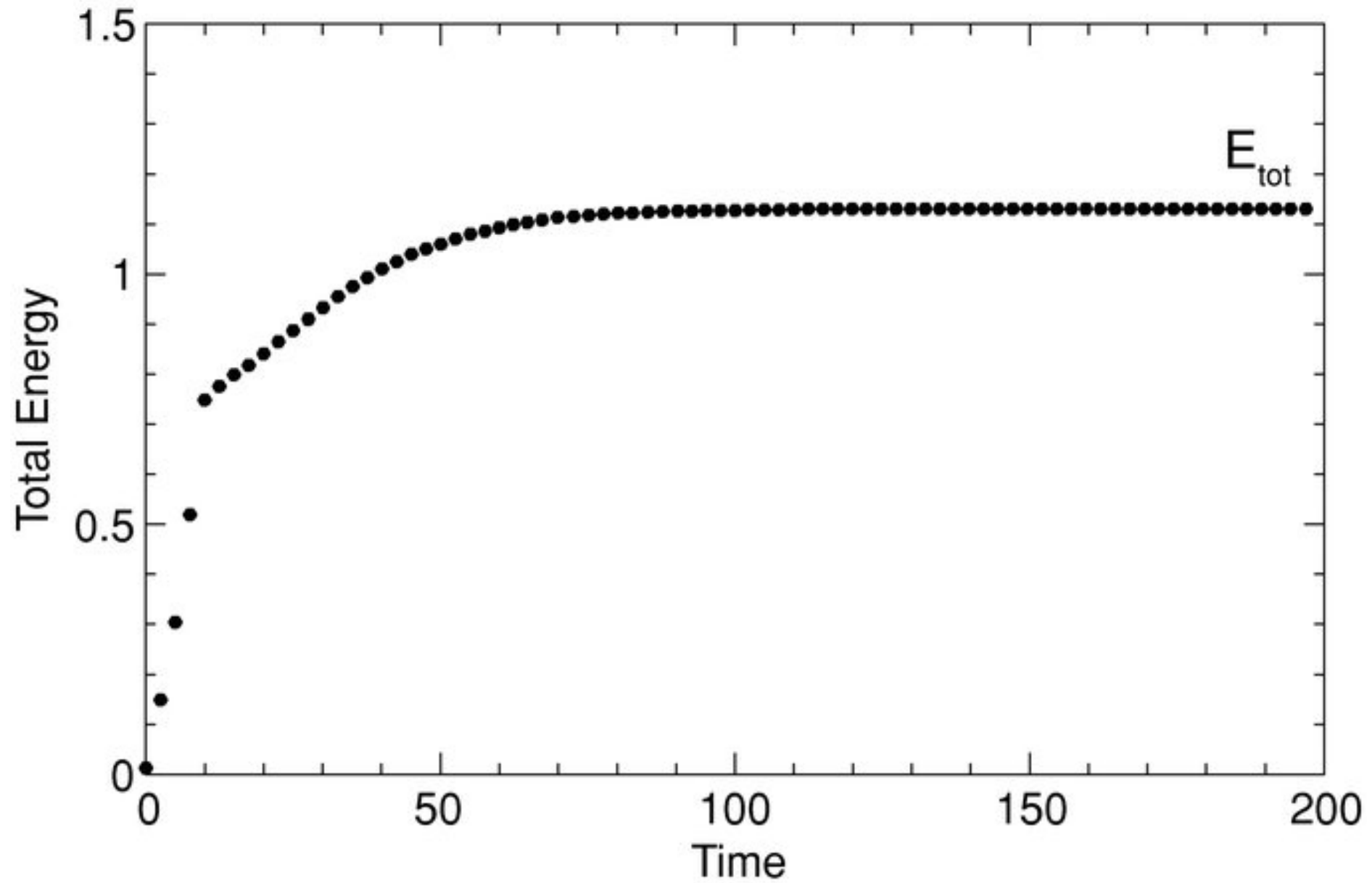
Figure 4. from How Does Radio AGN Feedback Feed Back? DE YOUNG 2010 ApJ 710 743 doi:10.1088/0004-637X/710/1/743 https://dx.doi.org/10.1088/0004-637X/710/1/743 © 2010. The American Astronomical Society. All rights reserved.
