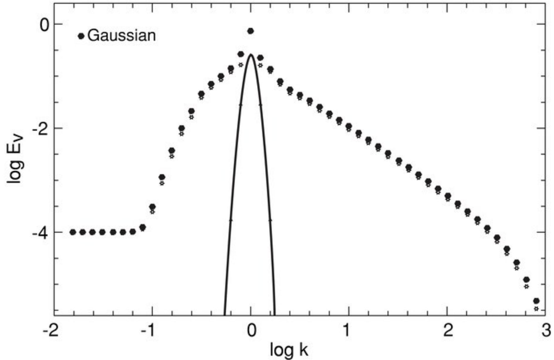
Figure 3. from How Does Radio AGN Feedback Feed Back? DE YOUNG 2010 ApJ 710 743 doi:10.1088/0004-637X/710/1/743 https://dx.doi.org/10.1088/0004-637X/710/1/743 © 2010. The American Astronomical Society. All rights reserved.
