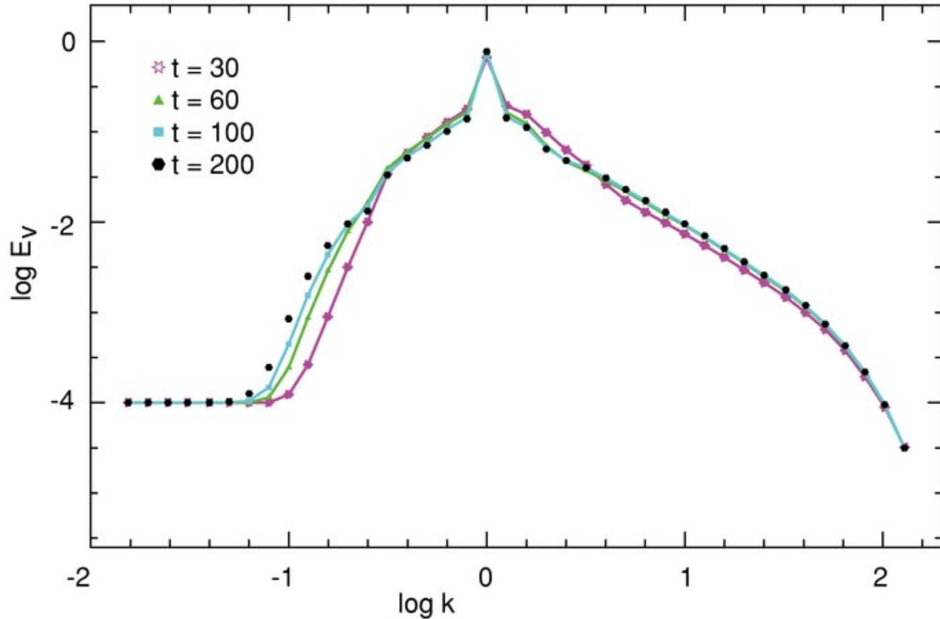
Figure 2. from How Does Radio AGN Feedback Feed Back? DE YOUNG 2010 ApJ 710 743 doi:10.1088/0004-637X/710/1/743 https://dx.doi.org/10.1088/0004-637X/710/1/743 © 2010. The American Astronomical Society. All rights reserved.
