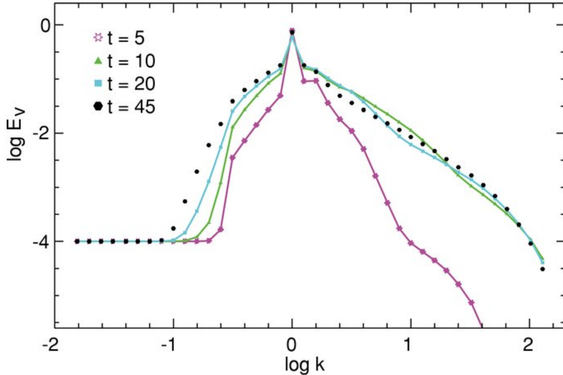
Figure 1. from How Does Radio AGN Feedback Feed Back? DE YOUNG 2010 ApJ 710 743 doi:10.1088/0004-637X/710/1/743 https://dx.doi.org/10.1088/0004-637X/710/1/743 © 2010. The American Astronomical Society. All rights reserved.
