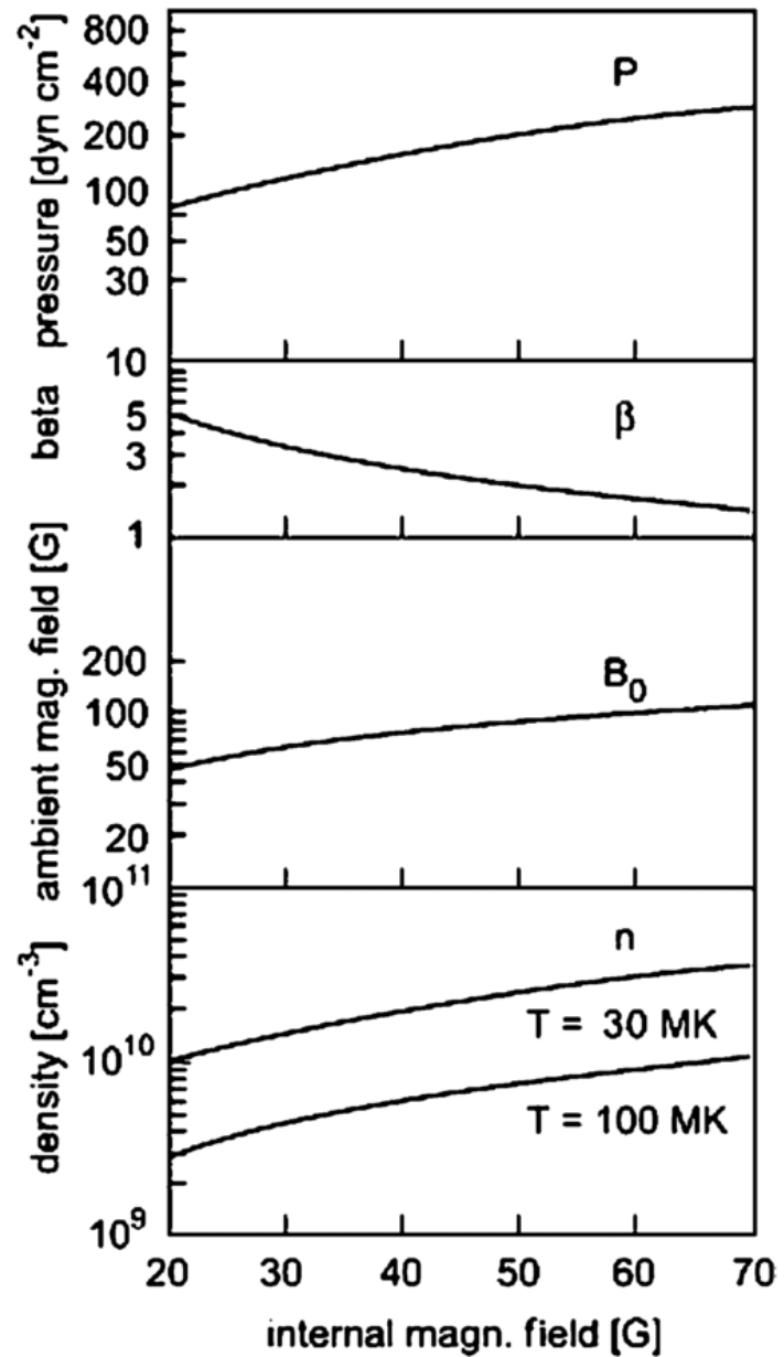
Figure 7. from Chromospheric Evaporation via Alfvén Waves HAERENDEL 2009 ApJ 707 903 doi:10.1088/0004-637X/707/2/903 https://dx.doi.org/10.1088/0004-637X/707/2/903 © 2009. The American Astronomical Society. All rights reserved.
