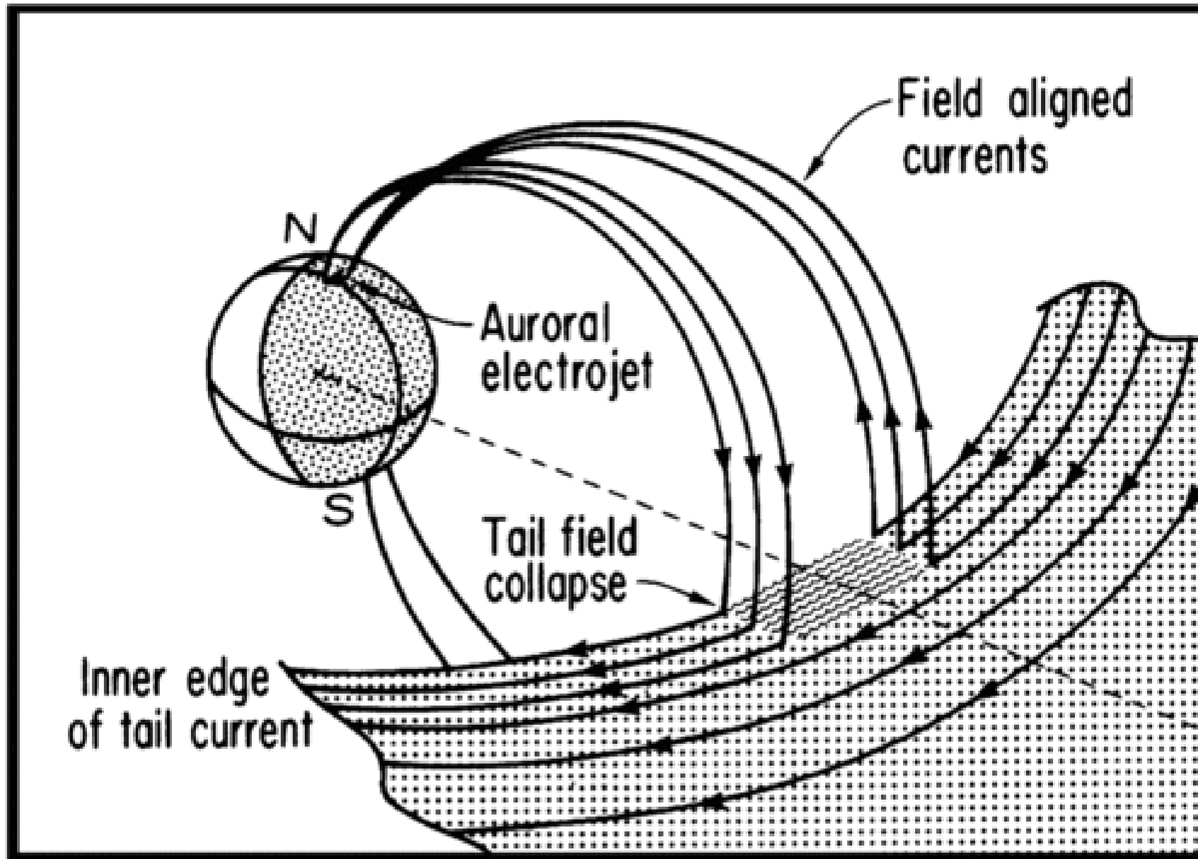
Figure 3. from Chromospheric Evaporation via Alfvén Waves HAERENDEL 2009 ApJ 707 903 doi:10.1088/0004-637X/707/2/903 https://dx.doi.org/10.1088/0004-637X/707/2/903 © 2009. The American Astronomical Society. All rights reserved.
