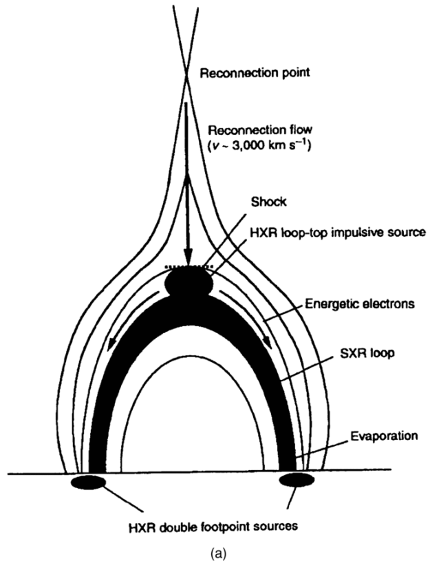
Figure 1. from Chromospheric Evaporation via Alfvén Waves HAERENDEL 2009 ApJ 707 903 doi:10.1088/0004-637X/707/2/903 https://dx.doi.org/10.1088/0004-637X/707/2/903 © 2009. The American Astronomical Society. All rights reserved.
