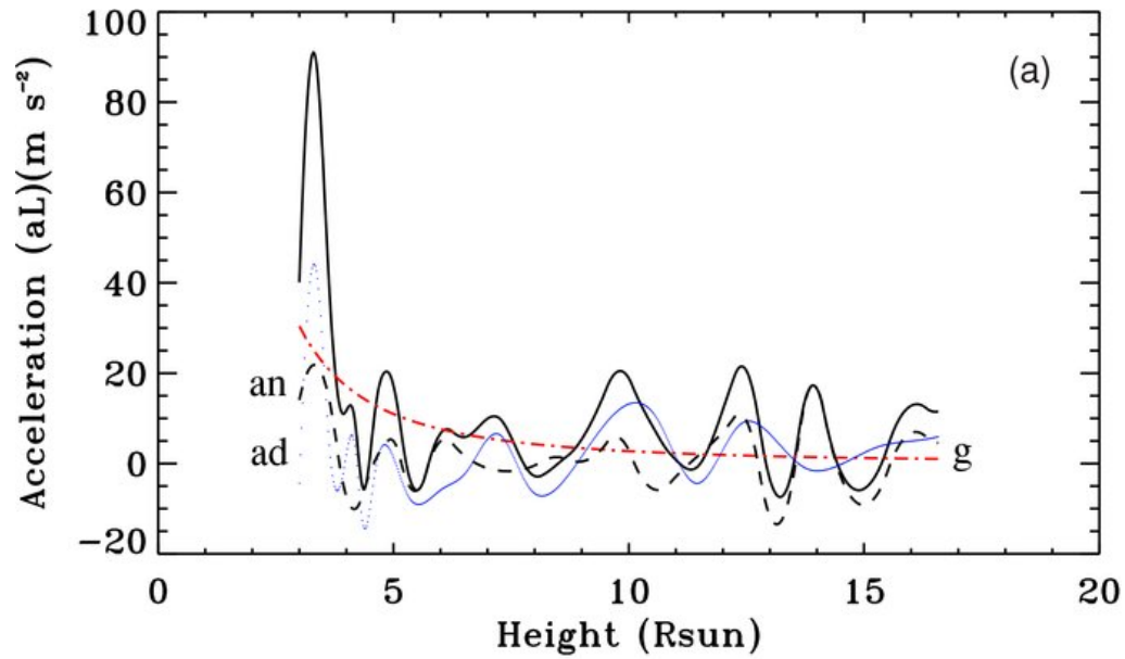
Figure 9. from Quasi-Periodic Oscillations in Lasco Coronal Mass Ejection Speeds SHANMUGARAJU ET AL. 2010 ApJ 708 450 doi:10.1088/0004-637X/708/1/450 https://dx.doi.org/10.1088/0004-637X/708/1/450
