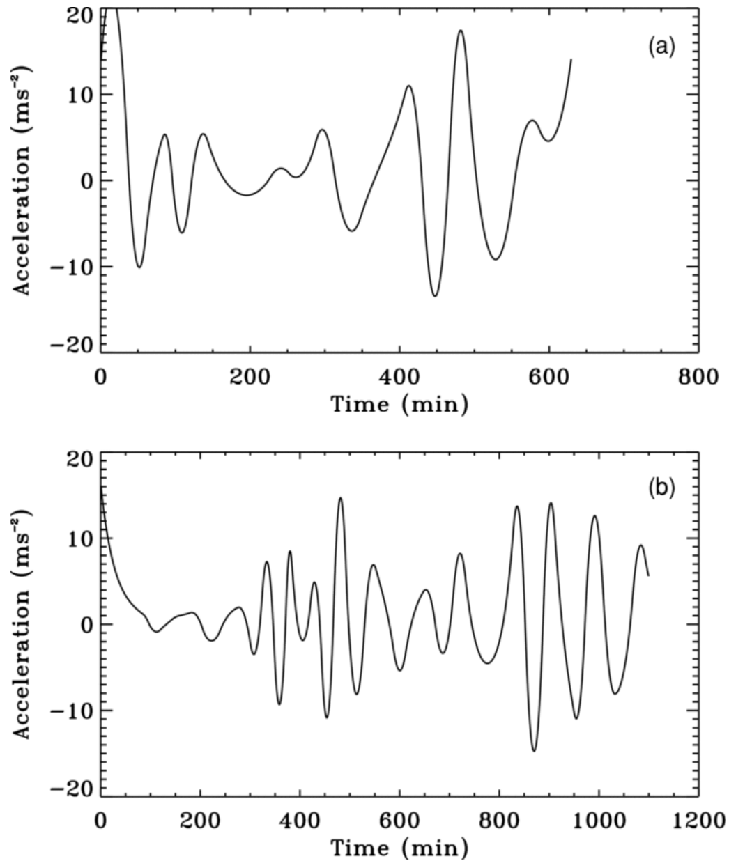
Figure 8. from Quasi-Periodic Oscillations in Lasco Coronal Mass Ejection Speeds SHANMUGARAJU ET AL. 2010 ApJ 708 450 doi:10.1088/0004-637X/708/1/450 https://dx.doi.org/10.1088/0004-637X/708/1/450
