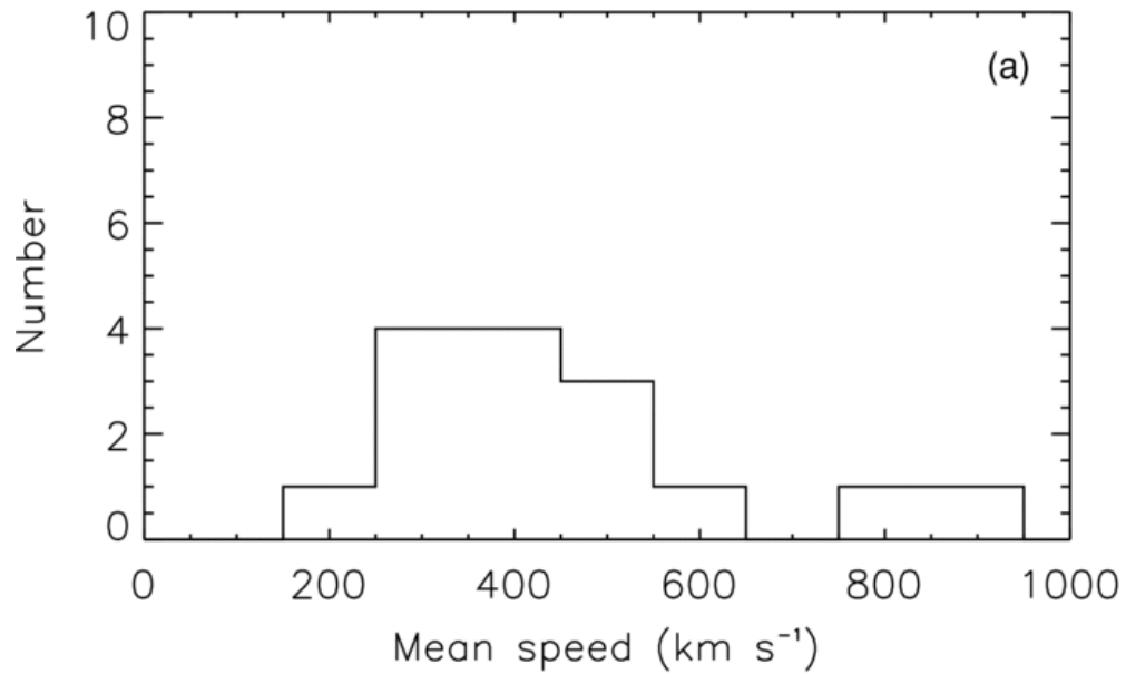
Figure 5. from Quasi-Periodic Oscillations in Lasco Coronal Mass Ejection Speeds SHANMUGARAJU ET AL. 2010 ApJ 708 450 doi:10.1088/0004-637X/708/1/450 https://dx.doi.org/10.1088/0004-637X/708/1/450
