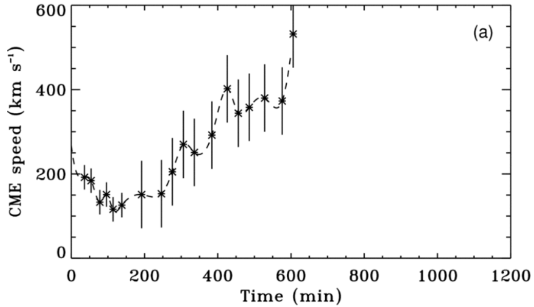
Figure 4. from Quasi-Periodic Oscillations in Lasco Coronal Mass Ejection Speeds SHANMUGARAJU ET AL. 2010 ApJ 708 450 doi:10.1088/0004-637X/708/1/450 https://dx.doi.org/10.1088/0004-637X/708/1/450
