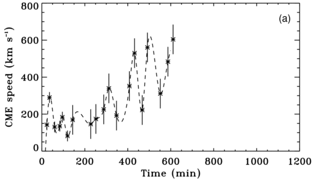
Figure 3. from Quasi-Periodic Oscillations in Lasco Coronal Mass Ejection Speeds SHANMUGARAJU ET AL. 2010 ApJ 708 450 doi:10.1088/0004-637X/708/1/450 https://dx.doi.org/10.1088/0004-637X/708/1/450
