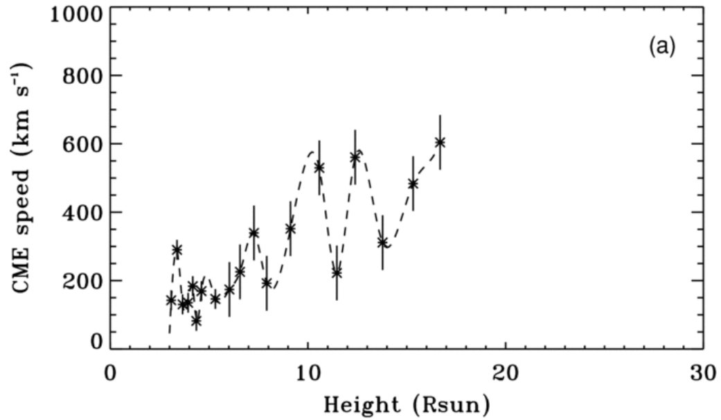
Figure 2. from Quasi-Periodic Oscillations in Lasco Coronal Mass Ejection Speeds SHANMUGARAJU ET AL. 2010 ApJ 708 450 doi:10.1088/0004-637X/708/1/450 https://dx.doi.org/10.1088/0004-637X/708/1/450
