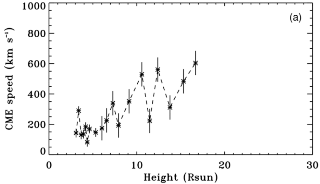
Figure 1. from Quasi-Periodic Oscillations in Lasco Coronal Mass Ejection Speeds SHANMUGARAJU ET AL. 2010 ApJ 708 450 doi:10.1088/0004-637X/708/1/450 https://dx.doi.org/10.1088/0004-637X/708/1/450
