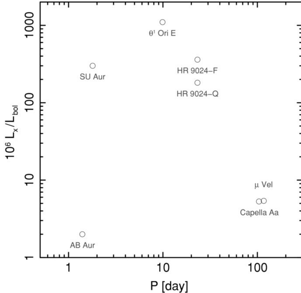
Figure 7. from X-Ray Emission and Corona of the Young Intermediate-Mass Binary 1 Ori E HUENEMOERDER ET AL. 2009 ApJ 707 942 doi:10.1088/0004-637X/707/2/942 https://dx.doi.org/10.1088/0004-637X/707/2/942 © 2009. The American Astronomical Society. All rights reserved.
