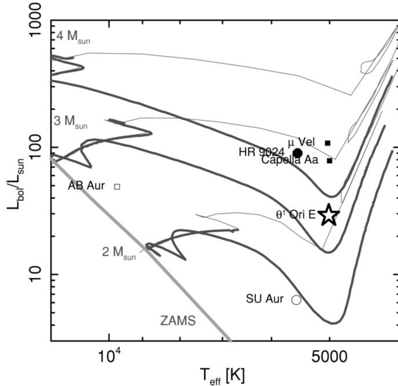
Figure 6. from X-Ray Emission and Corona of the Young Intermediate-Mass Binary 1 Ori E HUENEMOERDER ET AL. 2009 ApJ 707 942 doi:10.1088/0004-637X/707/2/942 https://dx.doi.org/10.1088/0004-637X/707/2/942 © 2009. The American Astronomical Society. All rights reserved.
