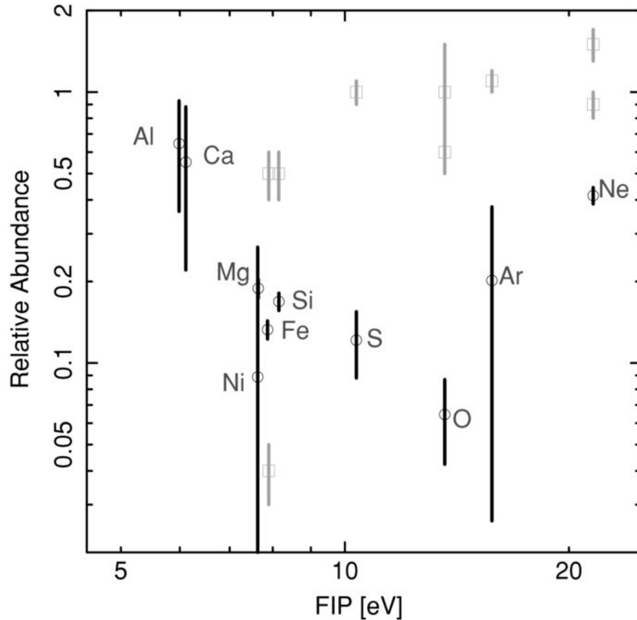
Figure 4. from X-Ray Emission and Corona of the Young Intermediate-Mass Binary 1 Ori E HUENEMOERDER ET AL. 2009 ApJ 707 942 doi:10.1088/0004-637X/707/2/942 https://dx.doi.org/10.1088/0004-637X/707/2/942 © 2009. The American Astronomical Society. All rights reserved.
