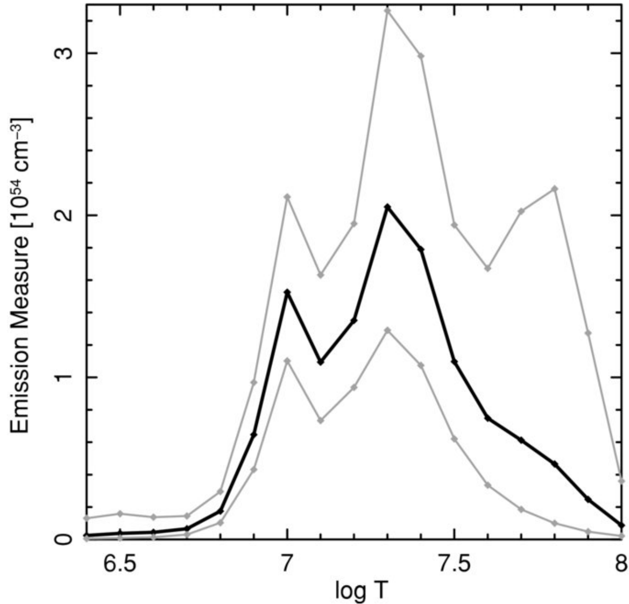
Figure 3. from X-Ray Emission and Corona of the Young Intermediate-Mass Binary 1 Ori E HUENEMOERDER ET AL. 2009 ApJ 707 942 doi:10.1088/0004-637X/707/2/942 https://dx.doi.org/10.1088/0004-637X/707/2/942 © 2009. The American Astronomical Society. All rights reserved.
