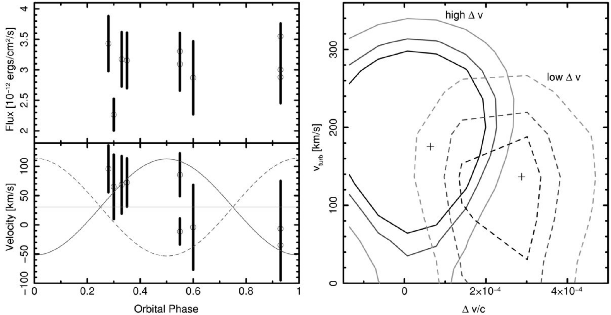
Figure 2. from X-Ray Emission and Corona of the Young Intermediate-Mass Binary 1 Ori E HUENEMOERDER ET AL. 2009 ApJ 707 942 doi:10.1088/0004-637X/707/2/942 https://dx.doi.org/10.1088/0004-637X/707/2/942 © 2009. The American Astronomical Society. All rights reserved.
