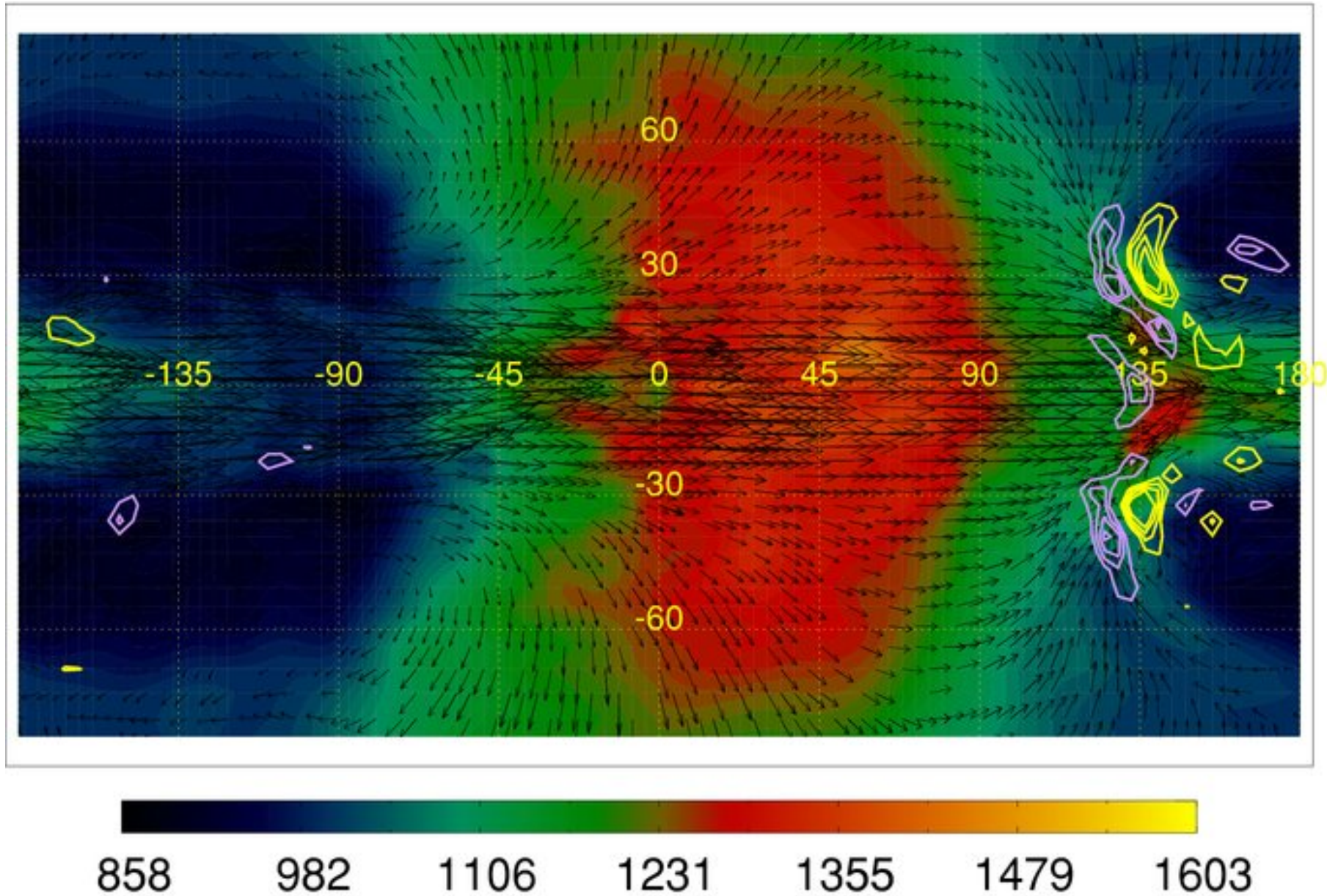
Figure 6. from Three-dimensional Modeling of Hot Jupiter Atmospheric Flows RAUSCHER & MENO 2010 ApJ 714 1334 doi:10.1088/0004-637X/714/2/1334 https://dx.doi.org/10.1088/0004-637X/714/2/1334 © 2010. The American Astronomical Society. All rights reserved.
