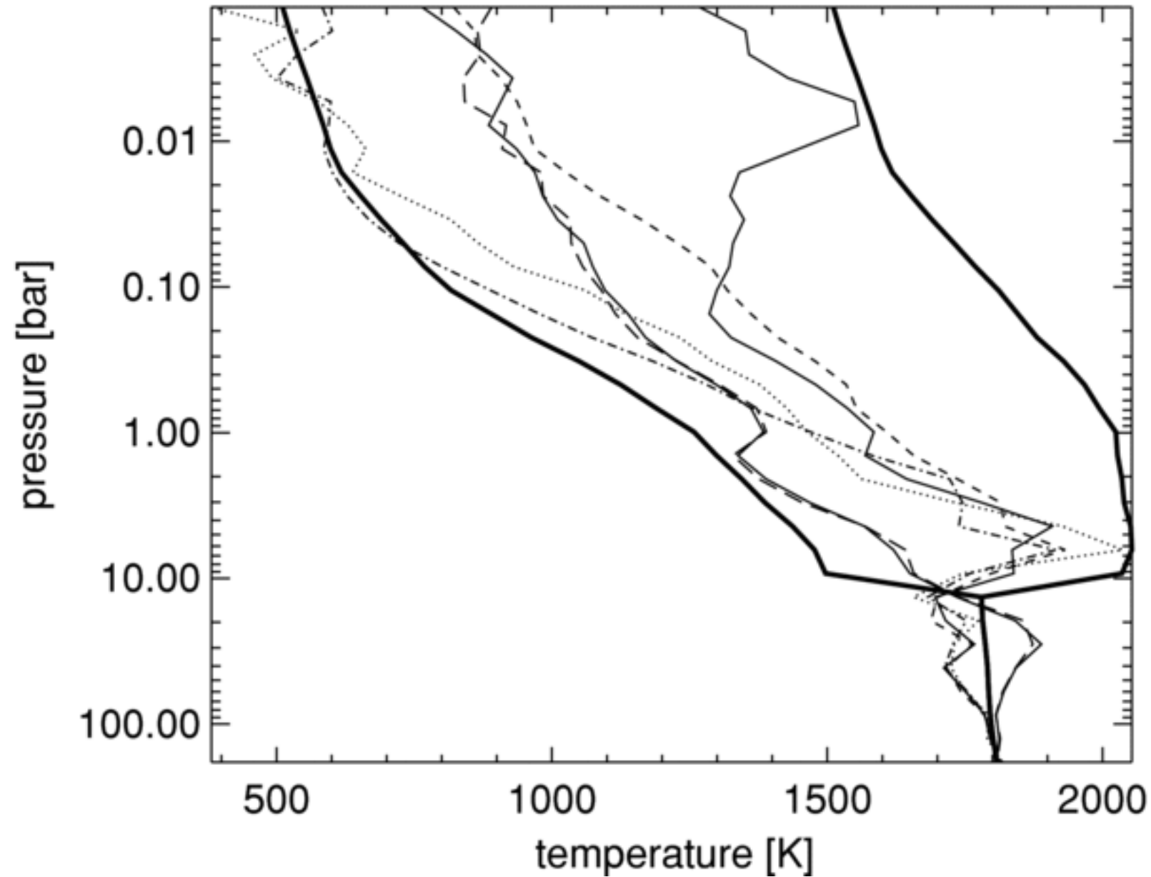
Figure 5. from Three-dimensional Modeling of Hot Jupiter Atmospheric Flows RAUSCHER & MENO 2010 ApJ 714 1334 doi:10.1088/0004-637X/714/2/1334 https://dx.doi.org/10.1088/0004-637X/714/2/1334 © 2010. The American Astronomical Society. All rights reserved.
