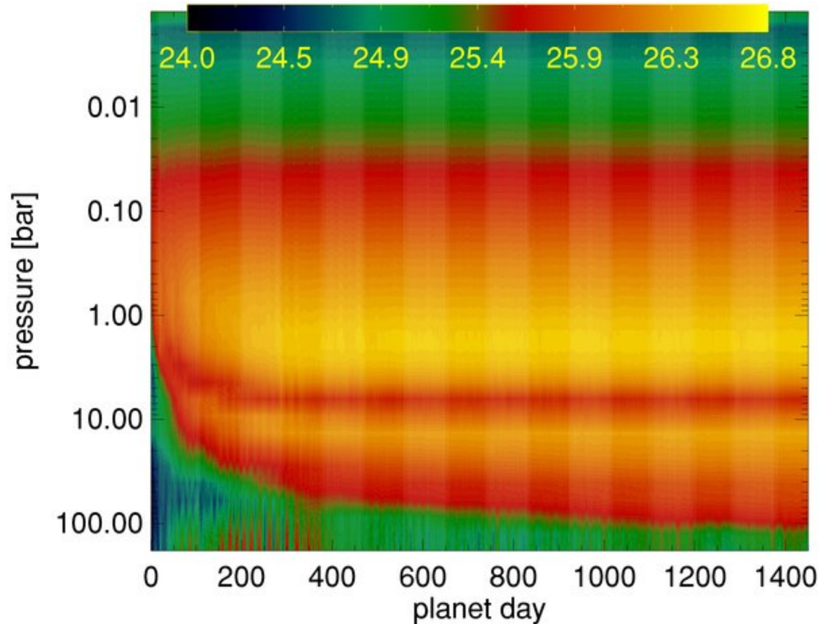
Figure 4. from Three-dimensional Modeling of Hot Jupiter Atmospheric Flows RAUSCHER & MENO 2010 ApJ 714 1334 doi:10.1088/0004-637X/714/2/1334 https://dx.doi.org/10.1088/0004-637X/714/2/1334 © 2010. The American Astronomical Society. All rights reserved.
