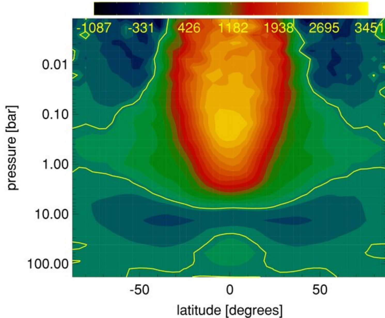
Figure 3. from Three-dimensional Modeling of Hot Jupiter Atmospheric Flows RAUSCHER & MENO 2010 ApJ 714 1334 doi:10.1088/0004-637X/714/2/1334 https://dx.doi.org/10.1088/0004-637X/714/2/1334 © 2010. The American Astronomical Society. All rights reserved.
