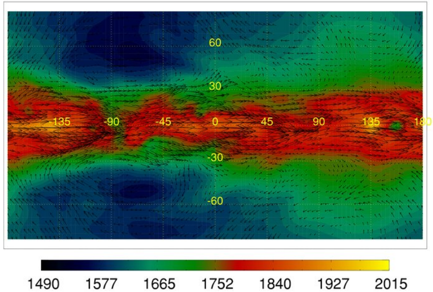
Figure 2. from Three-dimensional Modeling of Hot Jupiter Atmospheric Flows RAUSCHER & MENO 2010 ApJ 714 1334 doi:10.1088/0004-637X/714/2/1334 https://dx.doi.org/10.1088/0004-637X/714/2/1334 © 2010. The American Astronomical Society. All rights reserved.
