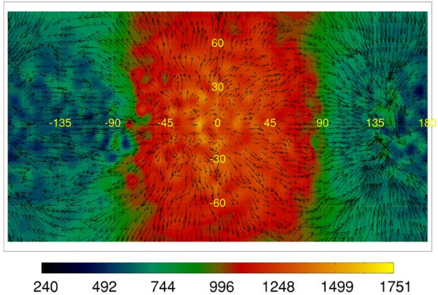
Figure 1. from Three-dimensional Modeling of Hot Jupiter Atmospheric Flows RAUSCHER & MENO 2010 ApJ 714 1334 doi:10.1088/0004-637X/714/2/1334 https://dx.doi.org/10.1088/0004-637X/714/2/1334 © 2010. The American Astronomical Society. All rights reserved.
